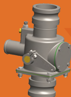
VÁLVULA BY PASS 2 1/2" AT 602/802 MACHO - MACHO (PADRÃO) 90015-MM
