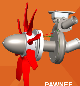
PAWNEE 01780-FA-X-8P-12V
