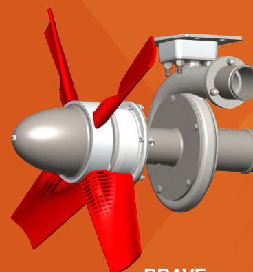
BRAVE 01640-BRAV-12V-X-6P
