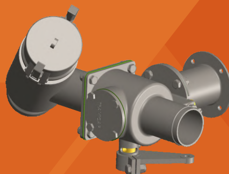
VÁLVULA BY PASS 2" IPANEMA FILTRO FLUXÔMETRO 01725H7-F
