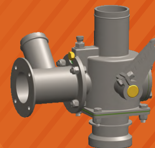
VÁLVULA BY PASS 2" CESSNA ON-OFF 01772H7-ONOFF
