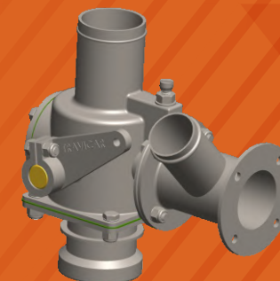
VÁLVULA BY PASS 2" IPANEMA ON-OFF 01725H7-ONOFF45
