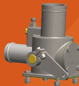
VÁLVULA BY PASS 2" AT 402/502 FLANGE - TUBO 01115-FLT
