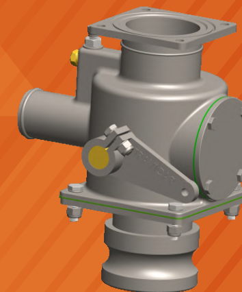
VÁLVULA BY PASS 2 1/2" AT 602/802 MACHO - FLANGE 2" 90015-MFL
