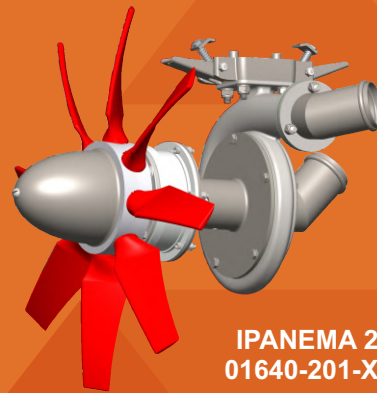
IPANEMA 202-203 01640-202/3-X-8P
